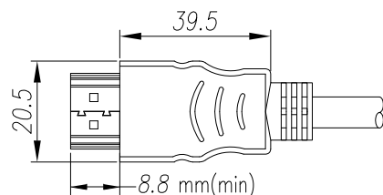
HDMI TYPE A MOLDING TYPE
