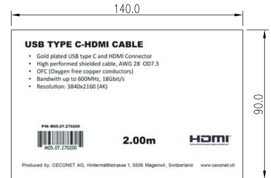
LABEL (1:2)
