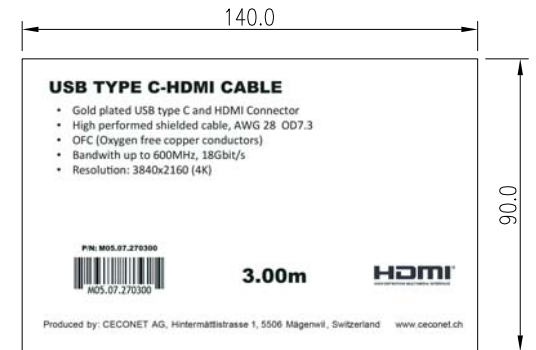
LABEL (1:2)
