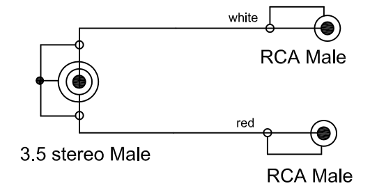
WIRING DIAGRAM
