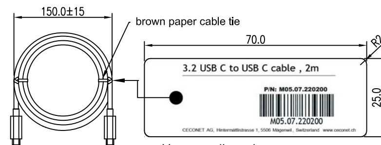
Hang cardboard
